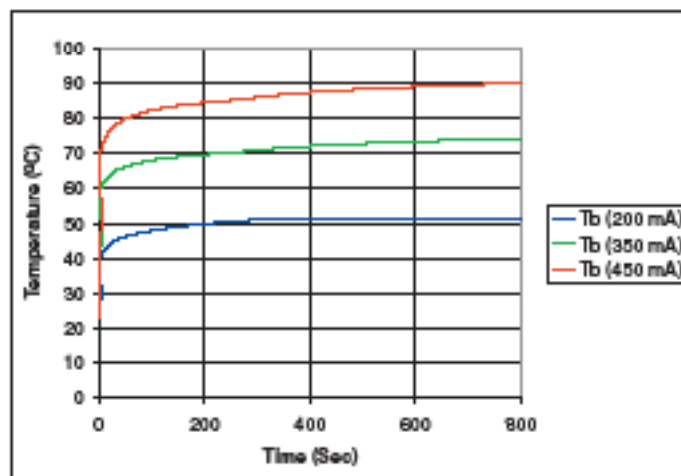
Figure 5: MCPCB Temperature
