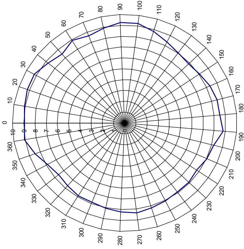
FWHM divergence versus side emitter rotation angle
