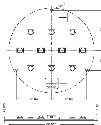
Flood Module
